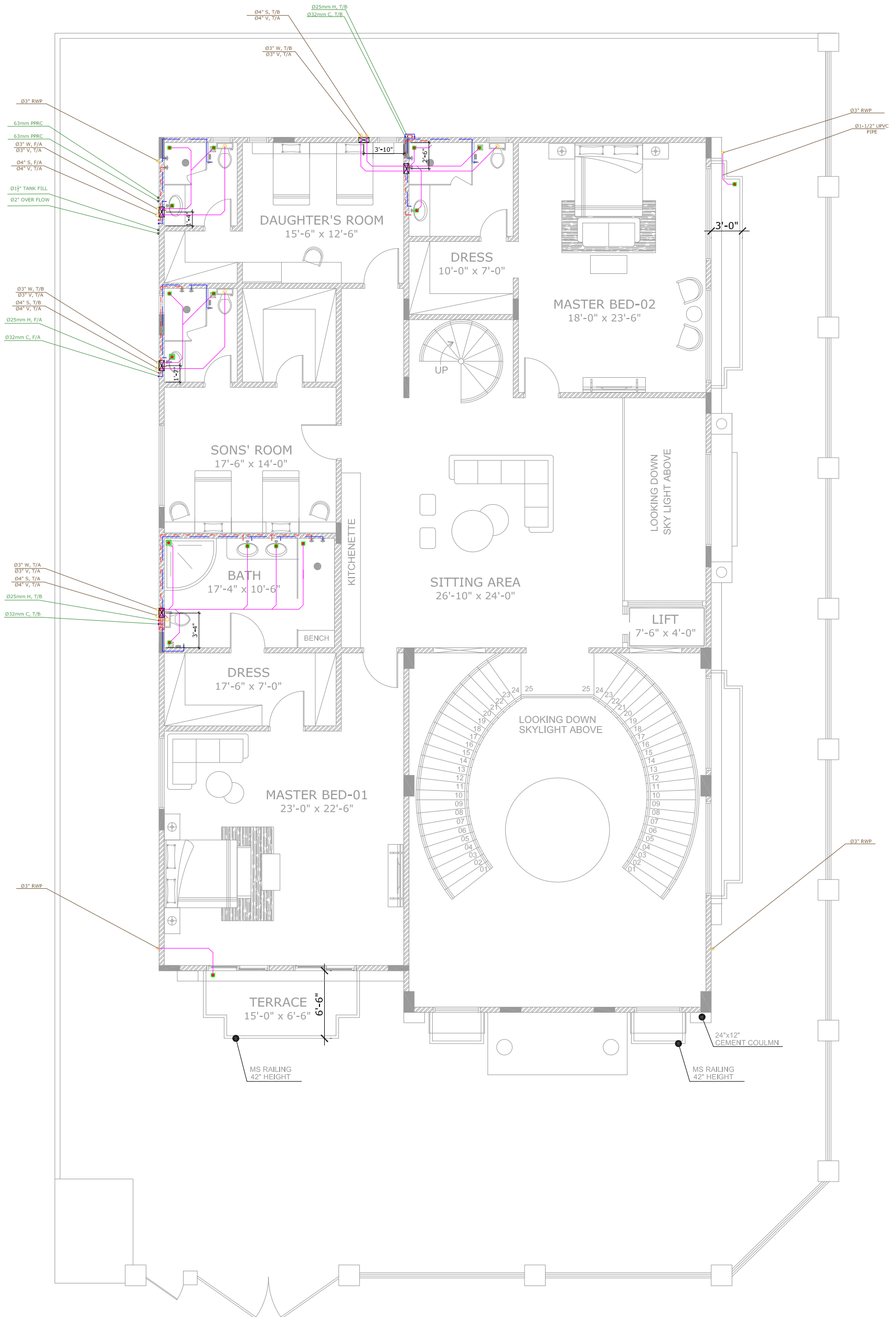
FIRST FLOOR SEWERAGE AND WATER SUPPLY | 1000 SQYD Residence Plumbing Layouts
