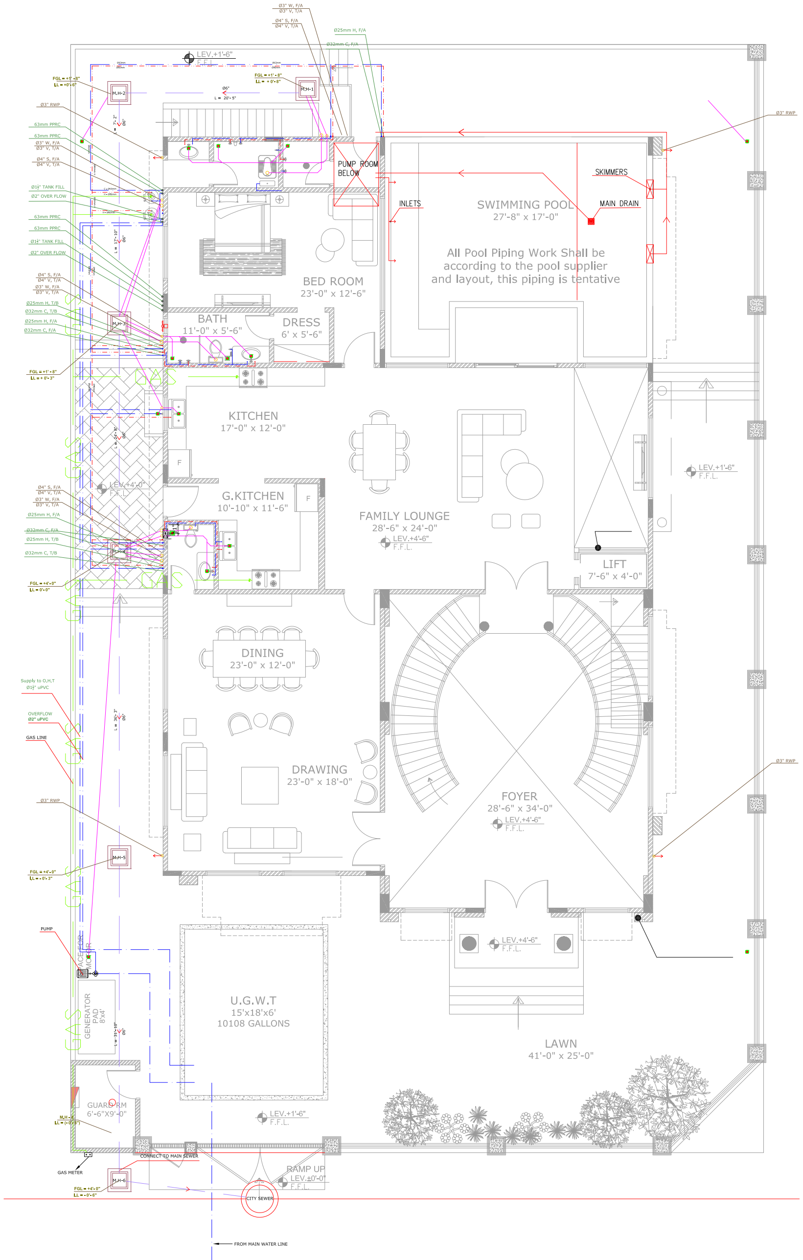
GROUND FLOOR SEWERAGE AND WATER SUPPLY | 1000 SQYD Residence Plumbing Layouts
